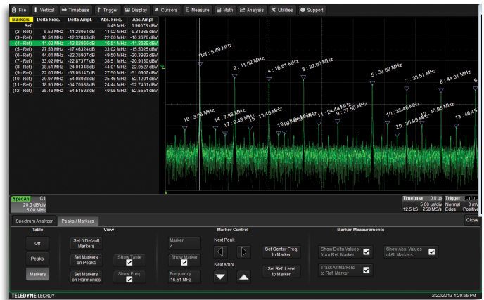
Spectrum Analyzer software uses oscilloscope channels, zooms, math functions or History Mode as source waveforms.
