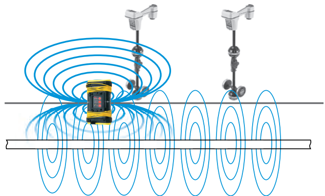
Figure 13 – Air Coupling
