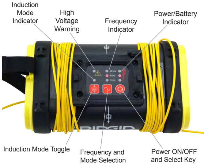
Figure 3 – Keypad and LED Indicators
